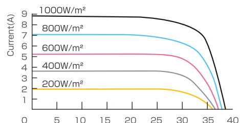
Current-Voltage Curve
